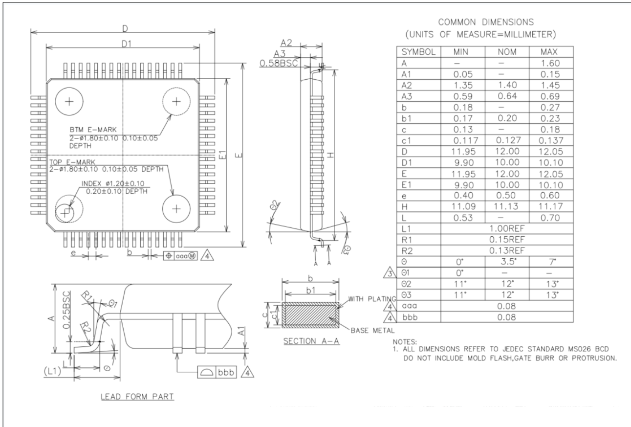
Figure 5-3 N32G052RBL7B package outline
