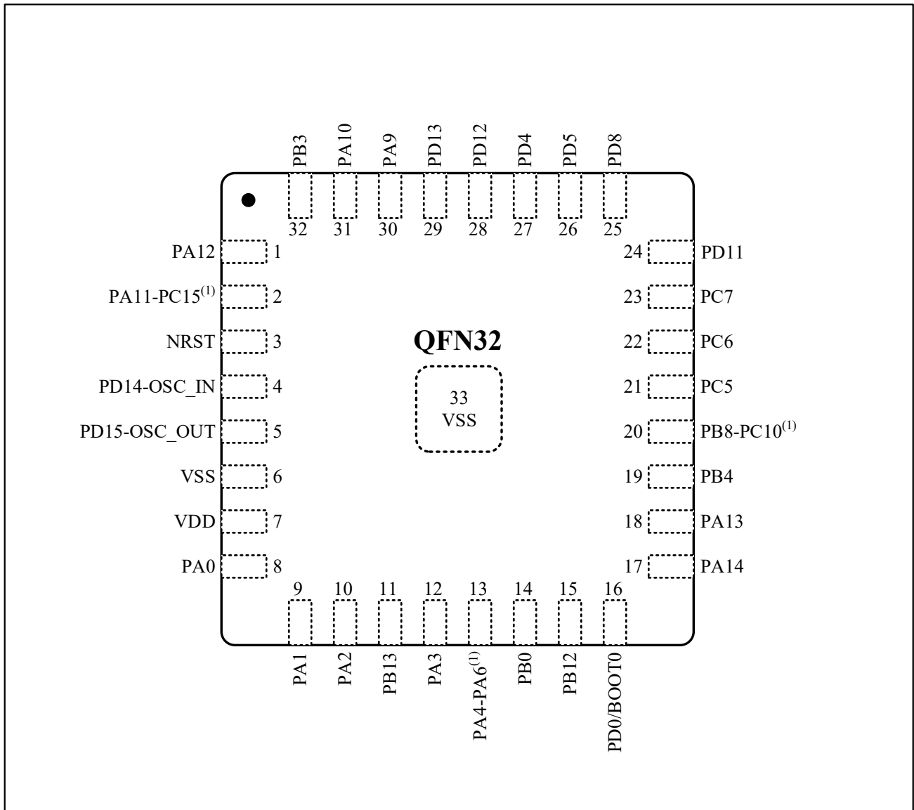
Figure 3-5 N32G052 Series QFN32 pinouts
