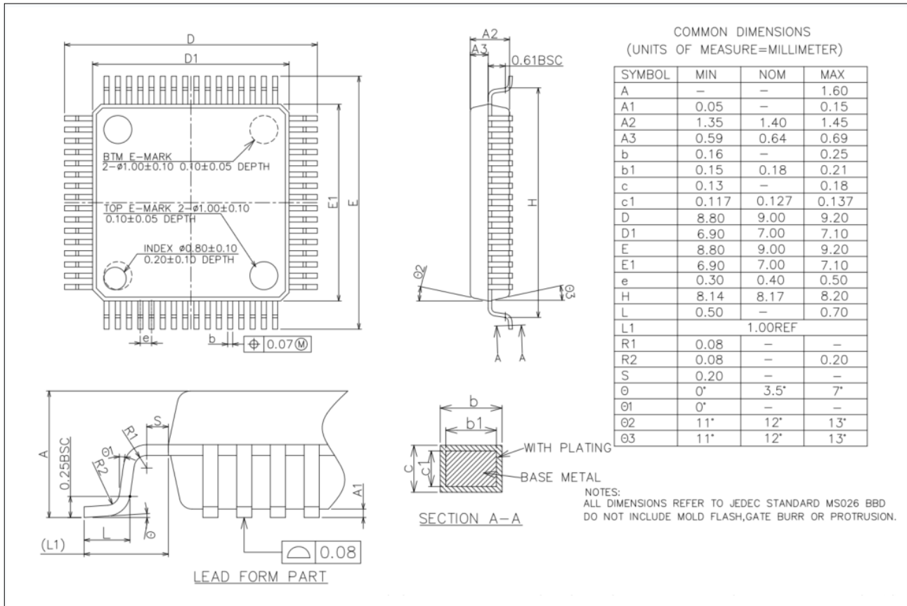
Figure 5-5 N32G052RBL7C package outline
