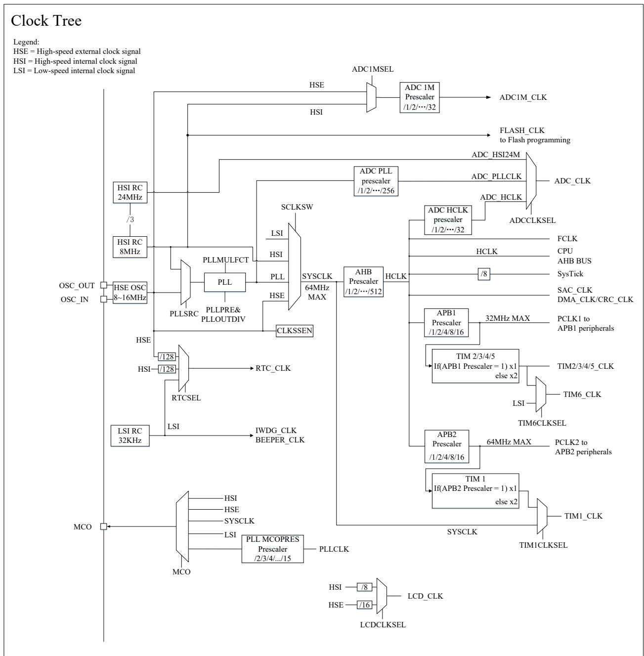
Figure 2-2 Clock Tree
