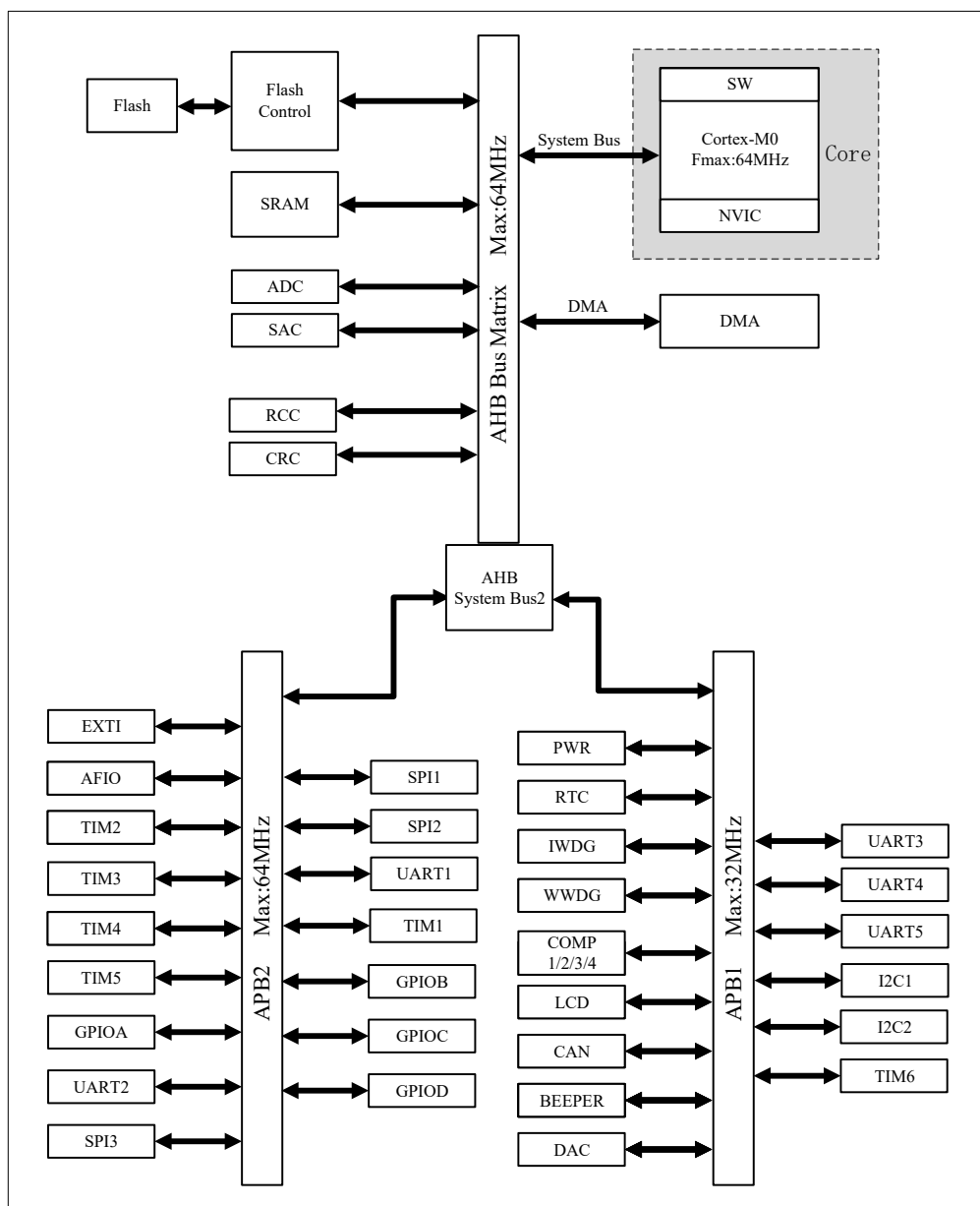
Figure 1-1 N32G052 Block Diagram
