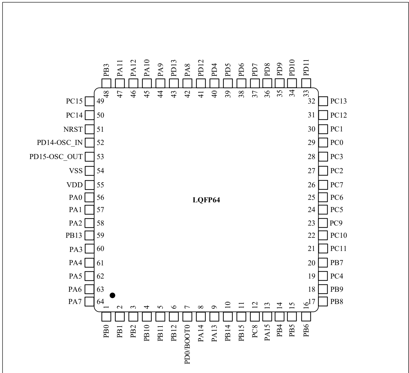
Figure 3-1 N32G052 Series LQFP64 pinouts
