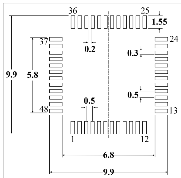
Figure 5-8 Suggestions for LQFP48 (7x7mm) package solder pads (1)
