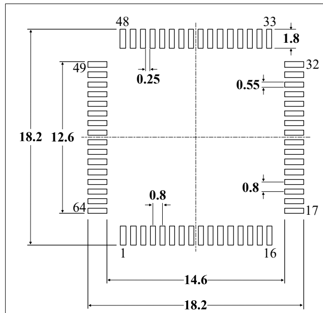
Figure 5-2 Suggestions for LQFP64 (14x14mm) package solder pads (1)
