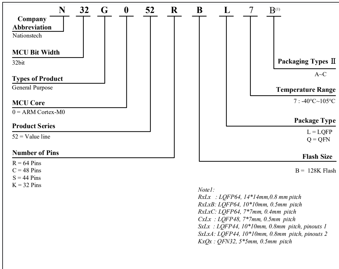
Figure 6-1 N32G052 series ordering code information diagram
