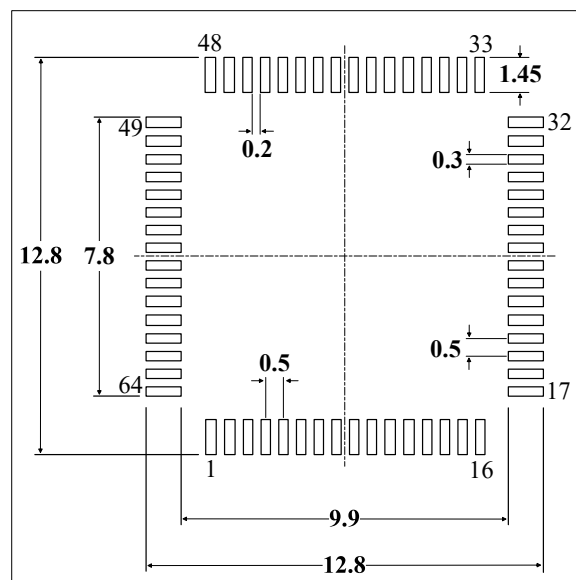
Figure 5-4 Suggestions for LQFP64 (10x10mm) package solder pads (1)
