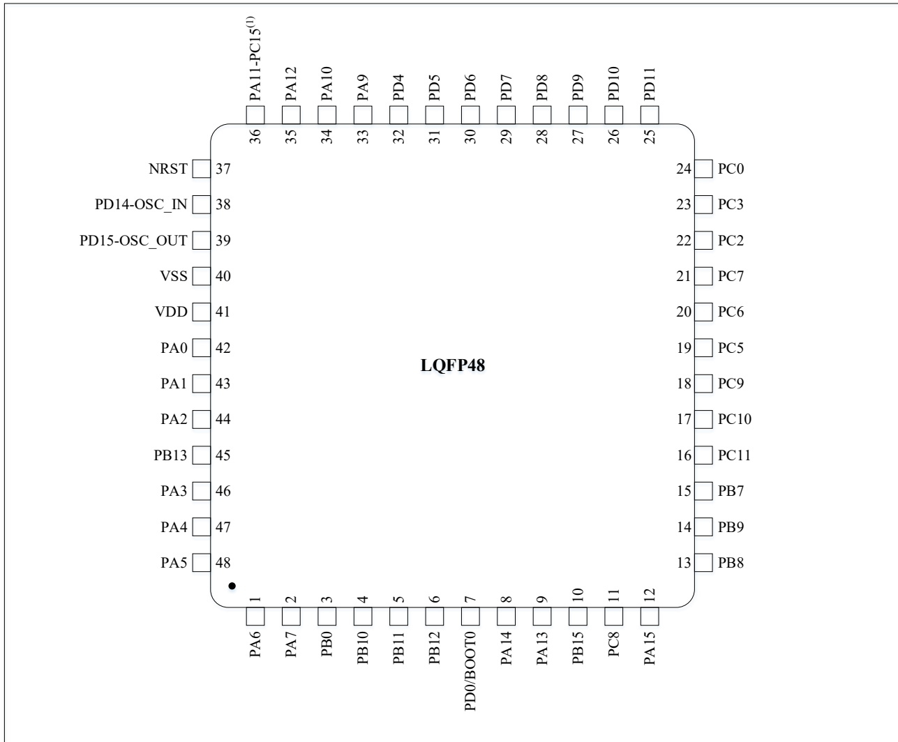
Figure 3-2 N32G052 Series LQFP48 pinouts
