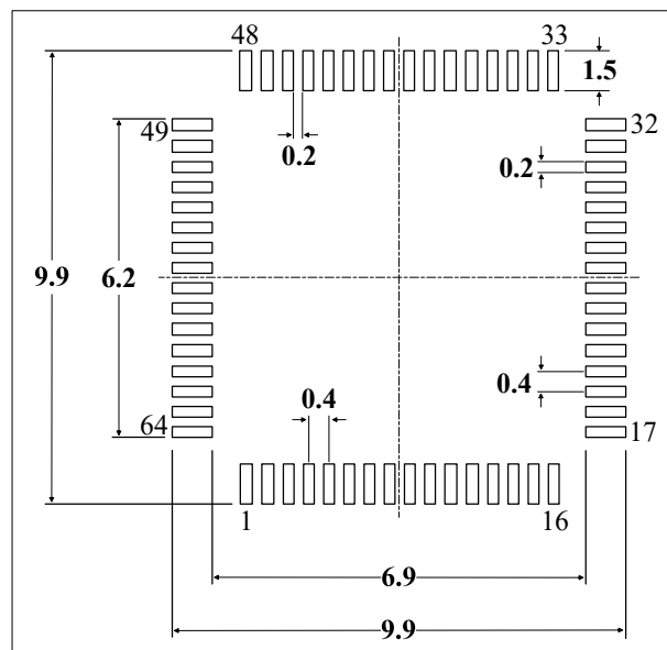
Figure 5-6 Suggestions for LQFP64 (7x7mm) package solder pads (1)
