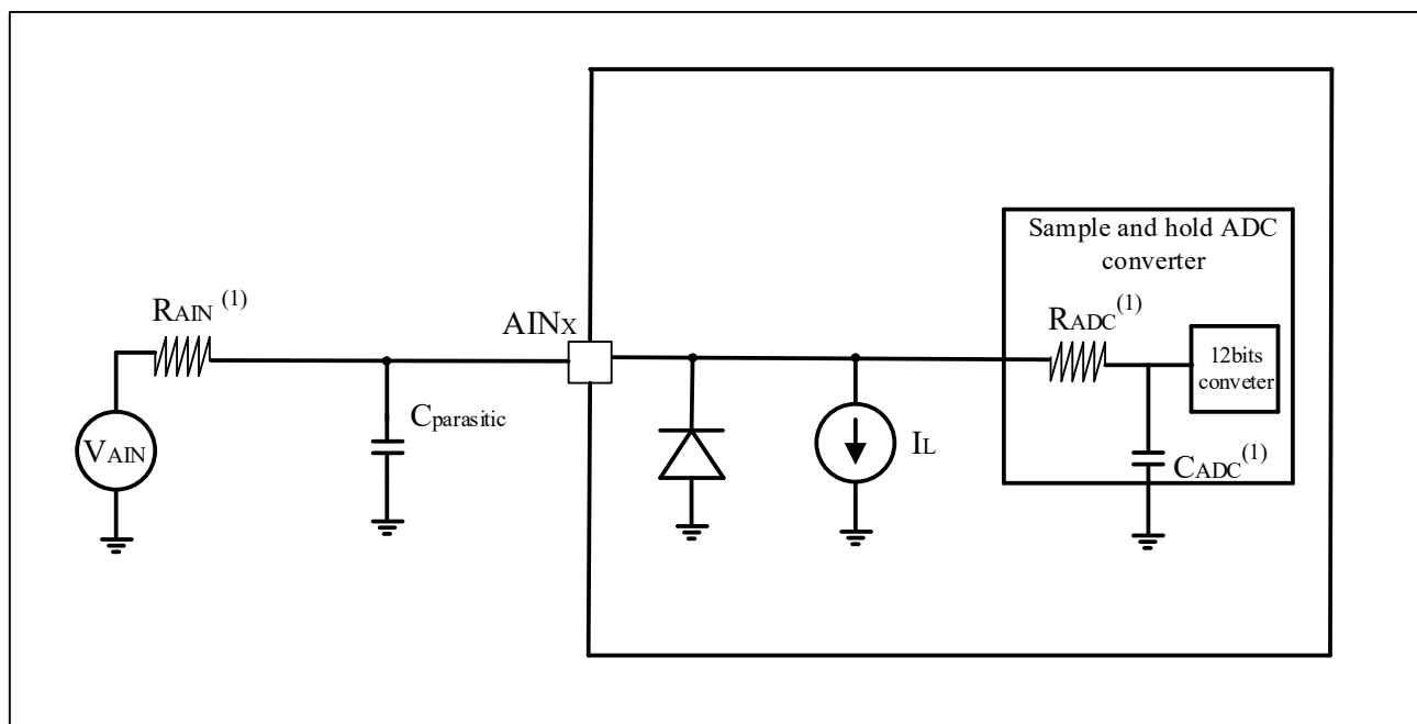
Figure 4-10 ADC typical connection diagram
