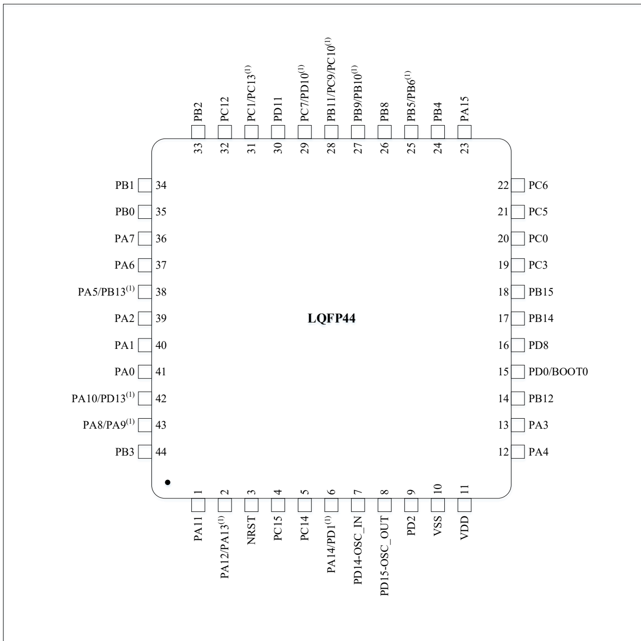
Figure 3-4 N32G052 Series LQFP44 pinouts 2
