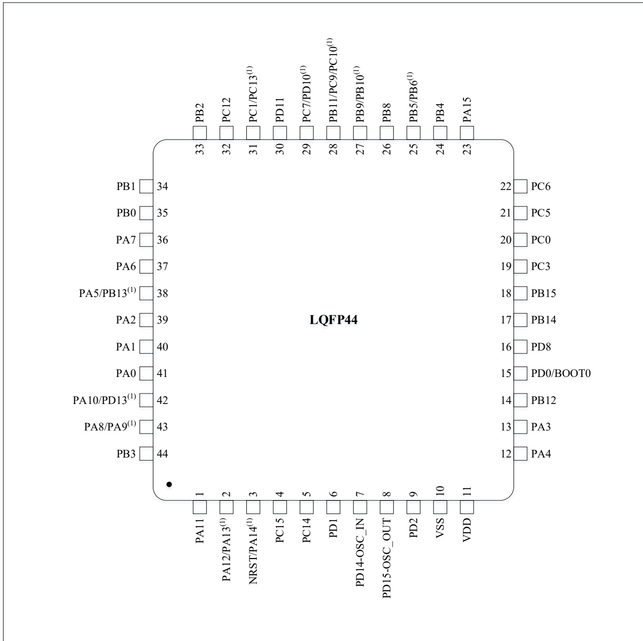
Figure 3-3 N32G052 Series LQFP44 pinouts 1
