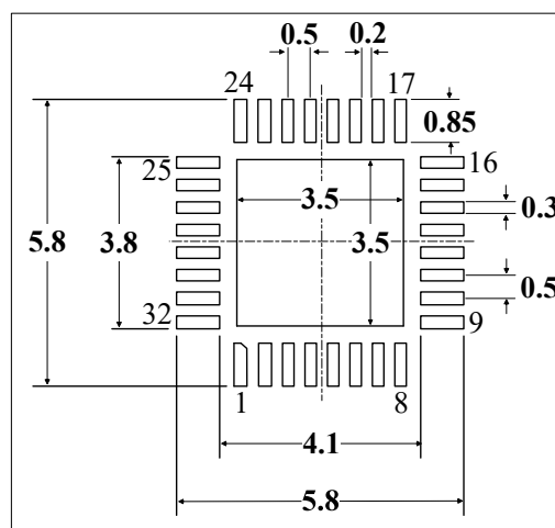
Figure 5-12 Suggestions for QFN32(5x5mm) package solder pads (1)
