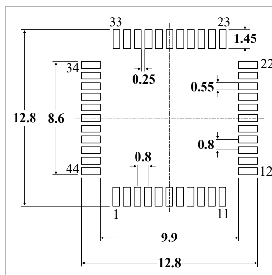
Figure 5-10 Suggestions for LQFP44(10x10mm) package solder pads (1)
